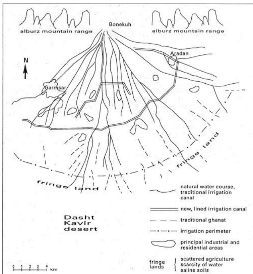
Figure 2. Sketch of the alluvial fan of Garmsar and its irrigation canal system.
