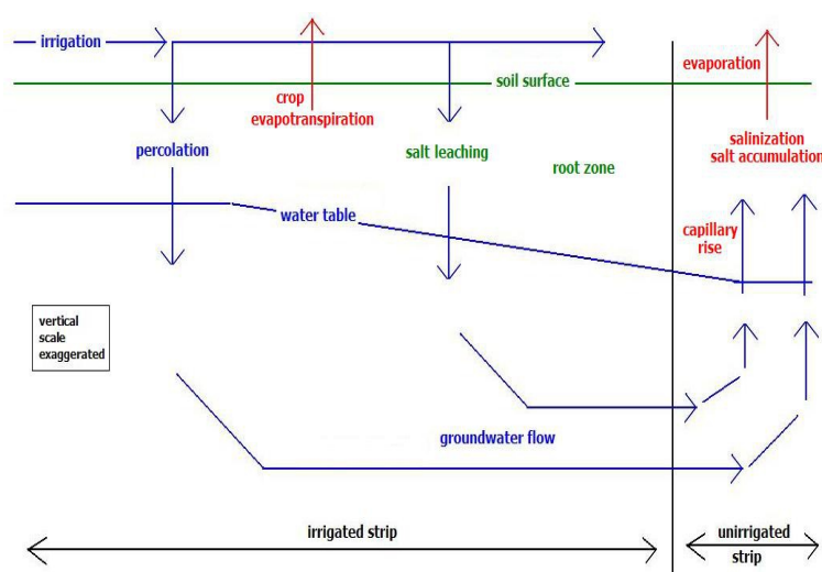
Principle of strip cropping with a sacrificial strip for salinity control in the cultivated strip
